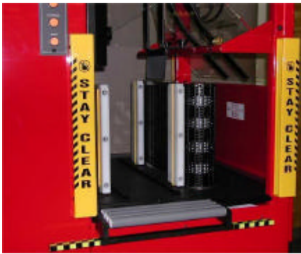
Quipp Light Curtain Safety Kits
